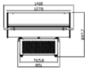
Vitrina inclinable Tilting display case
