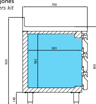
BMGN 1/3x100
