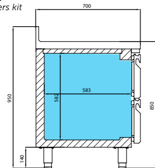
BMGN 1/2 x 200
